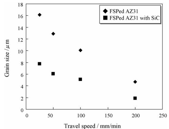
Fig. 7. Relationship between the grain size and the travel speed of the rotating tool.
